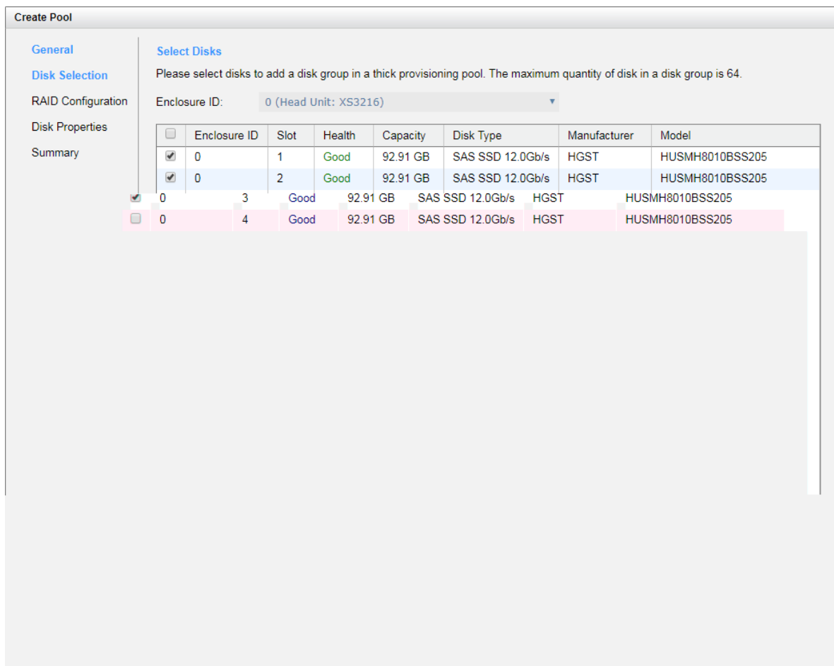
Figure 20 Create an SED Pool Step 2
