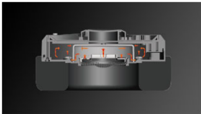
Dual-Chamber Design Speaker
