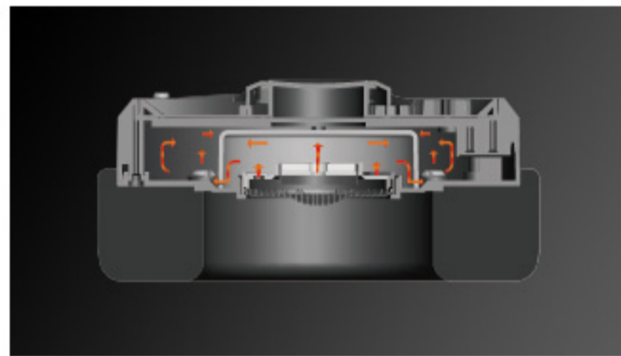
Dual-Chamber Design Speaker
